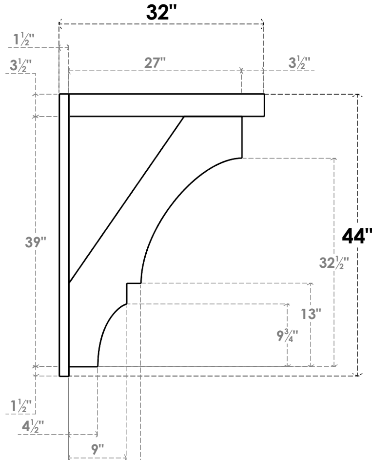
SIDE PROFILE
